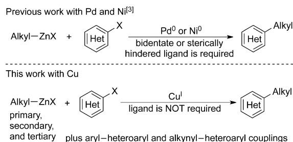
Scheme 3. Coupling of heteroaryl halides with alkylzinc reagents containing \beta -hydrogen atoms.
