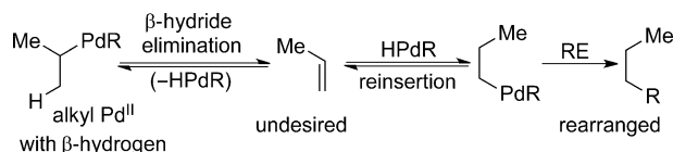
Scheme 1. Complications resulting from \beta -hydride elimination.
